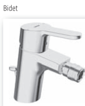
HANSAPRIMO one-hole single-lever basin mixer, DN 15 for bidet 4943 3203 chrome pop-up waste (metal), connection with flexible hoses G 3/8 projection: 107 mm
